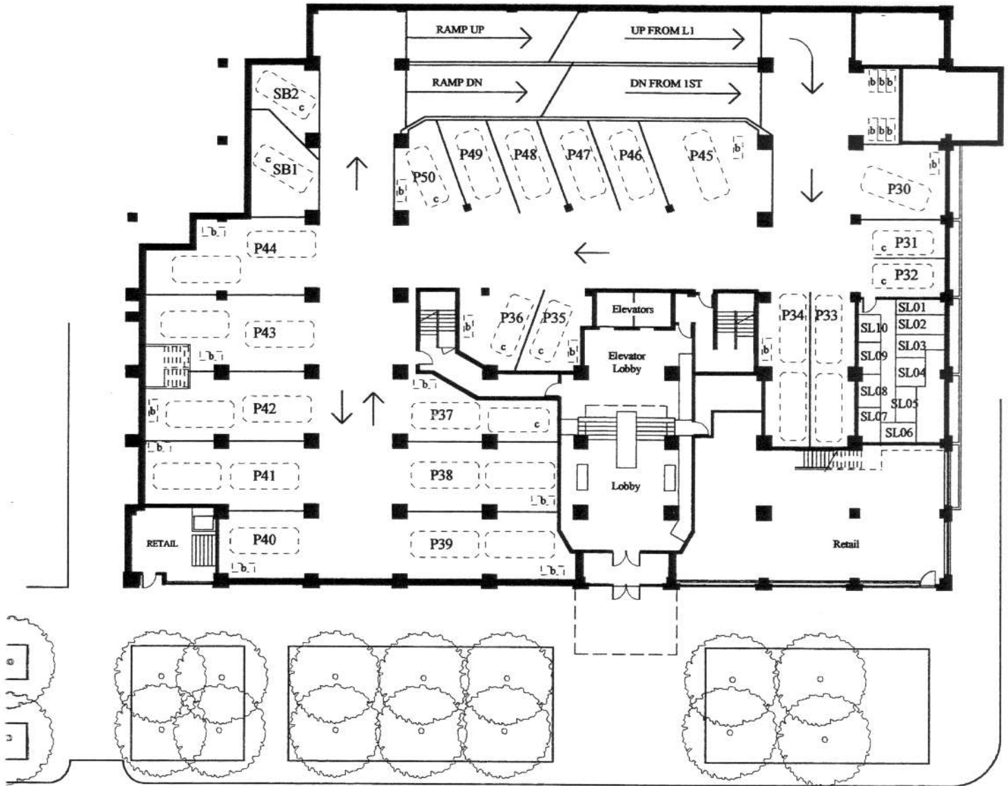
Lobby Level Plan
